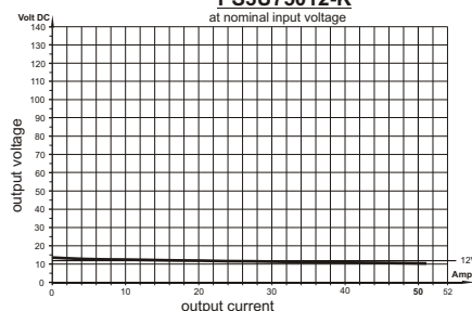
load diagram PS3U75012-K at nominal input voltage
