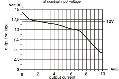
load diagram PSU10012 at nominal input voltage
