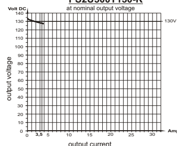
load diagram PS2U500T130-K
