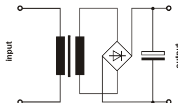
load diagram PS2U500T130-K
