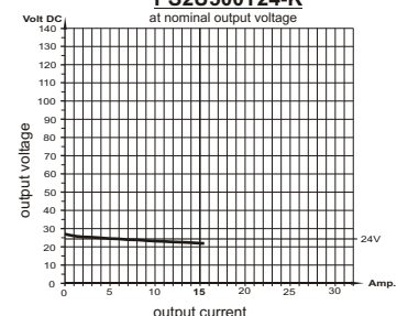
load diagram PS2U500T24-K at nominal output voltage
