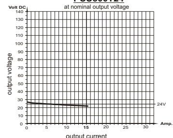
load diagram PSU500T24 at nominal output voltage
