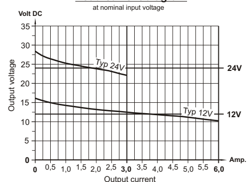
Load-current diagram
