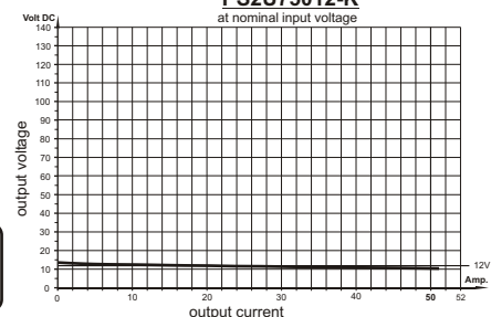
load diagram PS2U75012-K at nominal input voltage
