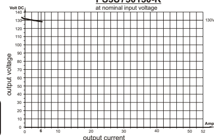
load diagram PS3U750130-K at nominal input voltage
