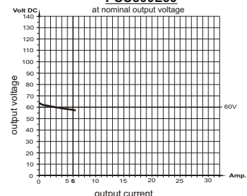
load diagram PSU500L60 at nominal output voltage
