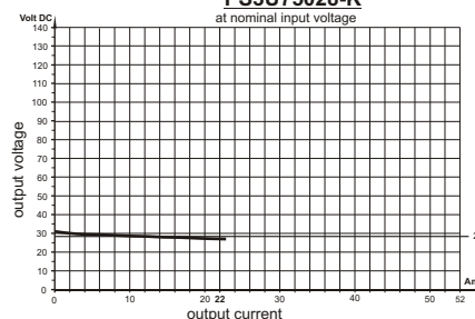
load diagram PS3U75028-K at nominal input voltage
