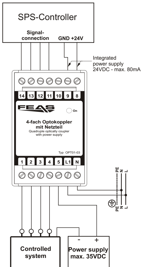
connection sample
