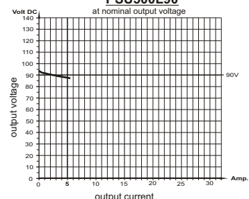
load diagram PSU500L90
