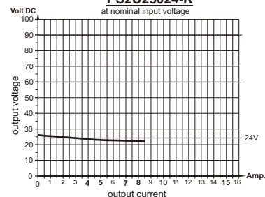
load diagram PS2U25024-K at nominal input voltage
