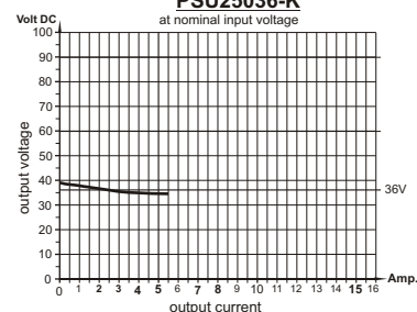
load diagram PSU25036-K at nominal input voltage
