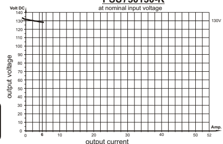
load diagram PSU750130-K at nominal input voltage
