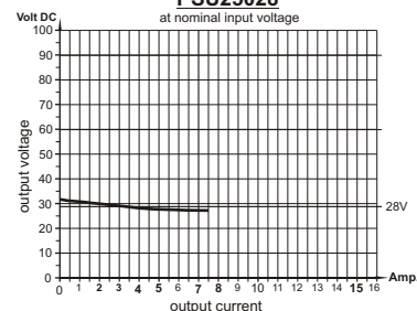
load diagram PSU25028 at nominal input voltage
