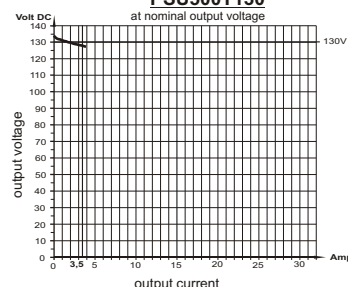
load diagram PSU500T130 at nominal output voltage
