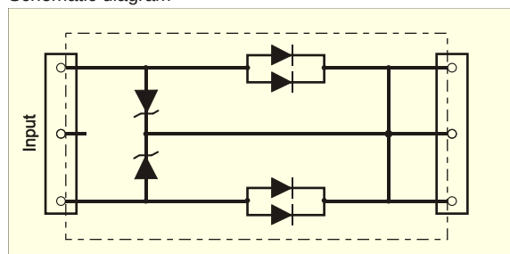
Schematic diagram
