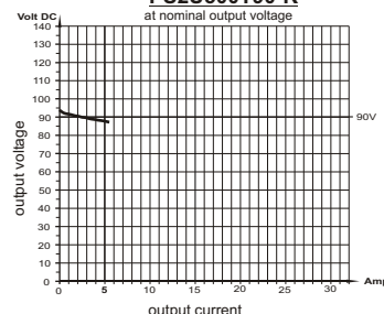
load diagram PS2U500T90-K at nominal output voltage
