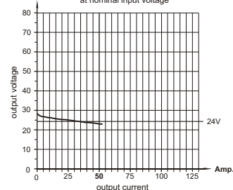
load diagram PS5U1K224-K at nominal input voltage
