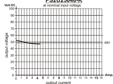
load diagram PS2U25048-K at nominal input voltage
