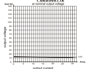
load diagram PS2U500T12 at nominal output voltage
