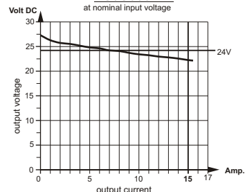
load diagram PS5U500T24 at nominal input voltage
