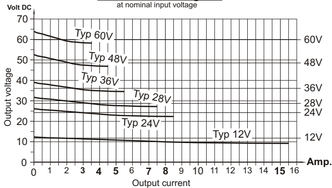
Load current diagram at nominal input voltage
