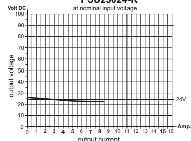
load diagram PSU25024-K at nominal input voltage
