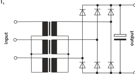
load diagram PS5U75024
