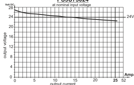
load diagram PS5U75024
