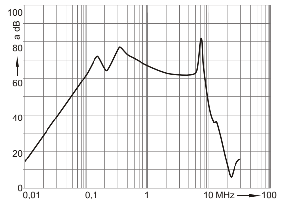
Insertion loss at 50
