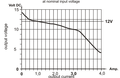
load diagram PSLC122 at nominal input voltage
