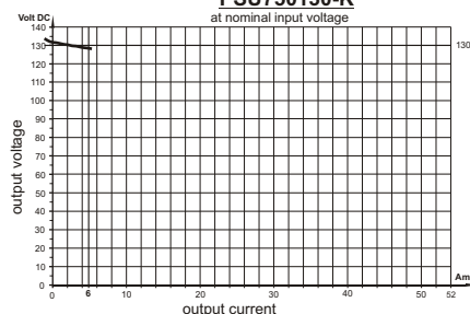
load diagram PSU750130-K at nominal input voltage
