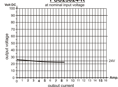
load diagram PSU25024-K at nominal input voltage
