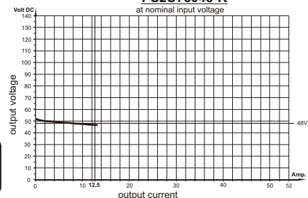
load diagram PS2U75048-K at nominal input voltage
