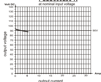
load diagram PS2U500L90-K at nominal input voltage
