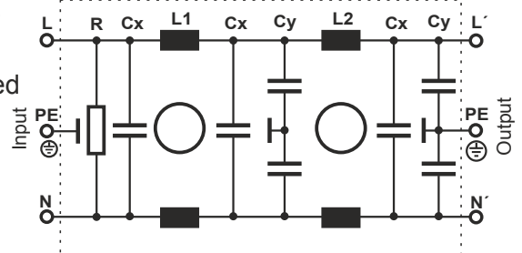
typical connection scheme optimised against asymmetric interferences
