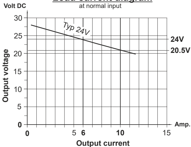
Load current diagram at normal input
