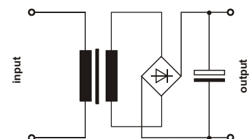
load diagram PSU18012
