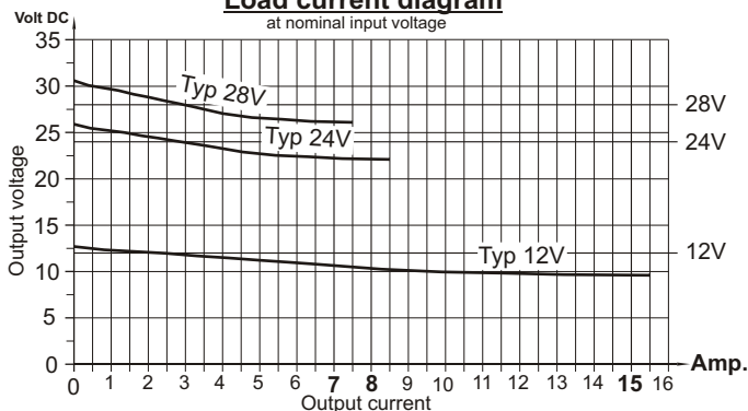
Load current diagram at nominal input voltage
