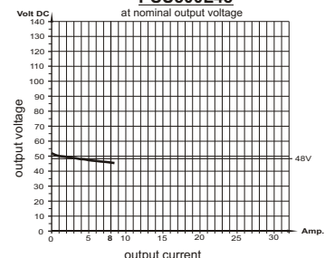
load diagram PSU500L48 at nominal output voltage
