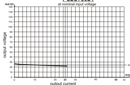
load diagram PS2U75024 at nominal input voltage
