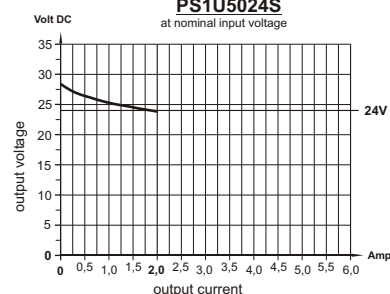
load diagram PS1U5024S at nominal input voltage
