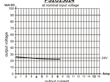
load diagram PS2U25024 at nominal input voltage
