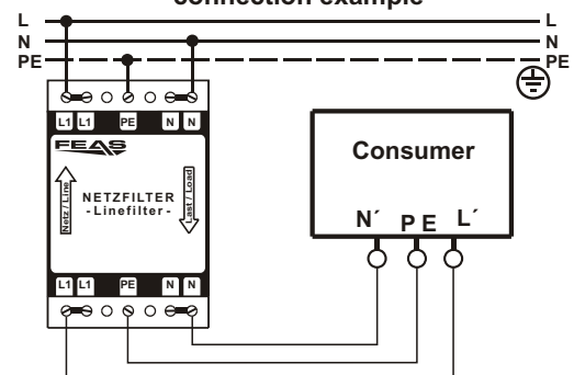
connection example
