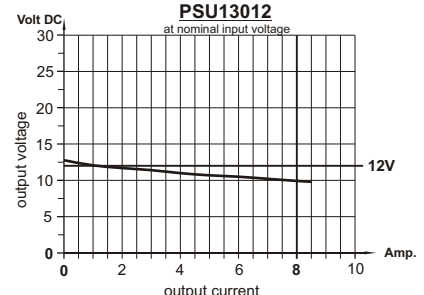
load diagram PSU13012 at nominal input voltage
