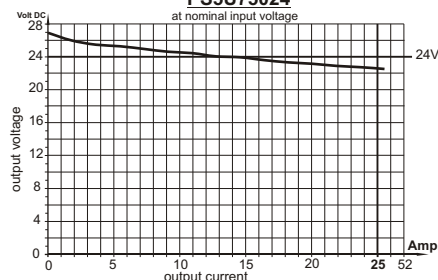
load diagram PS5U75024 at nominal input voltage
