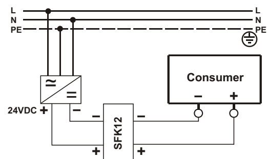
connection example
