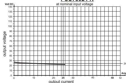
load diagram PSU75024-K at nominal input voltage
