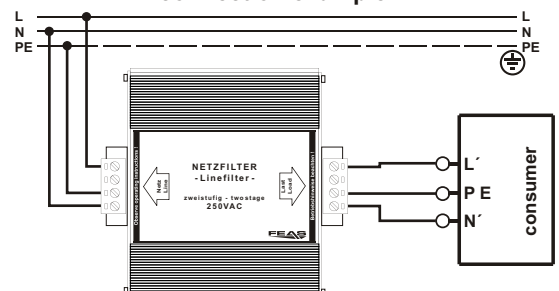
connection example
