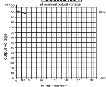
load diagram PSU500L130-K at nominal output voltage
