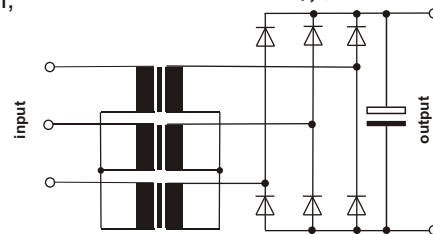
load diagram
