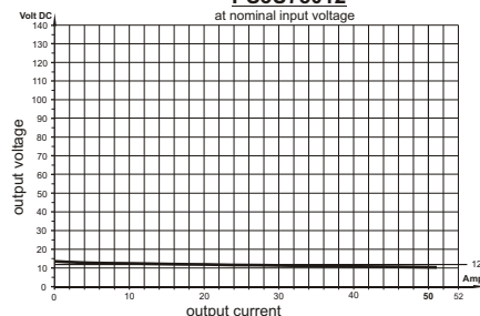
load diagram
