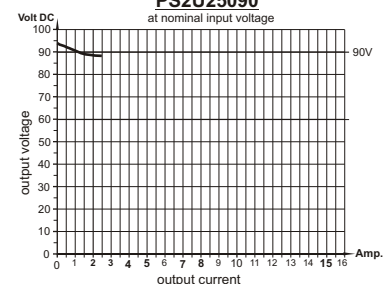
load diagram PS2U25090 at nominal input voltage
