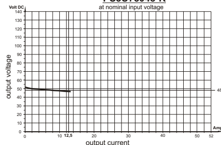
load diagram PS3U75048-K at nominal input voltage
